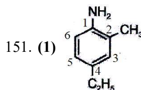
4-Ethyl-2-methylaniline
